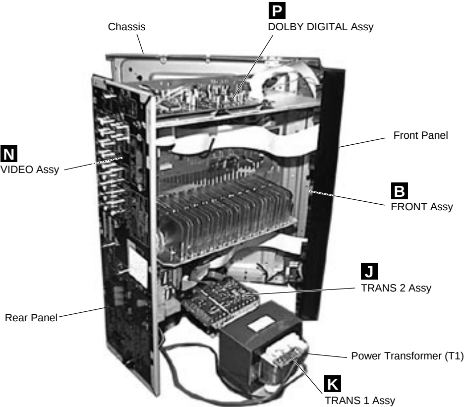
Rear View
